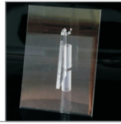
Plug-in holder DIN A4, pre-assembled with 2 clips, for Light-Sticks 75-190 cm, approx. w 21 x h 29,7 x d 12 cm. Item no.: WLZB011
